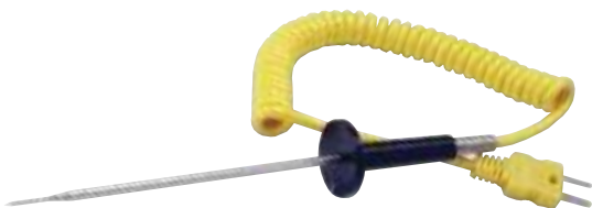
9817 Step down penetration probe with 1.575mm tip diameter and 3' lead.
