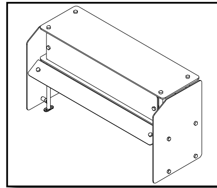
DCFSHG Series Double tier display bottom tier sneezeguard style, second tier full glass front
