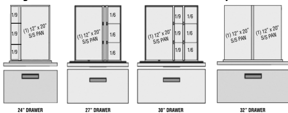
Drawer configurations for UCD4400N/UCD4500N Series only.
