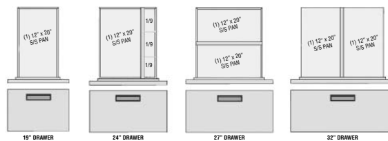
Drawer configurations for BUCM and BSTM series.
