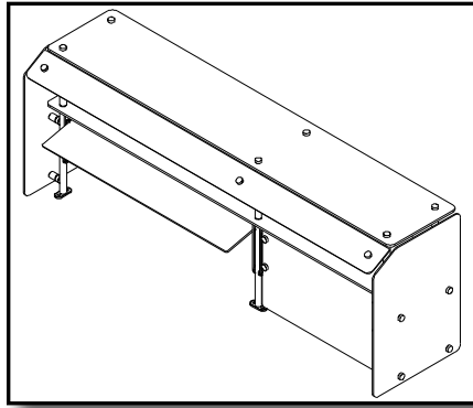
DCFSFS2 Series Double tier flexible foodshield (pivots in three positions)
